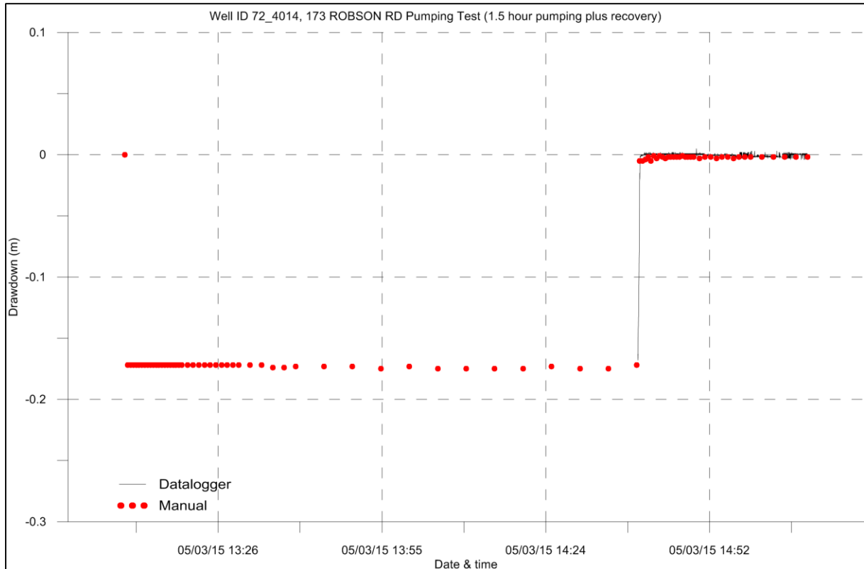
Figure A 3.9 Drawdown and recovery plot for well 72_4014.
