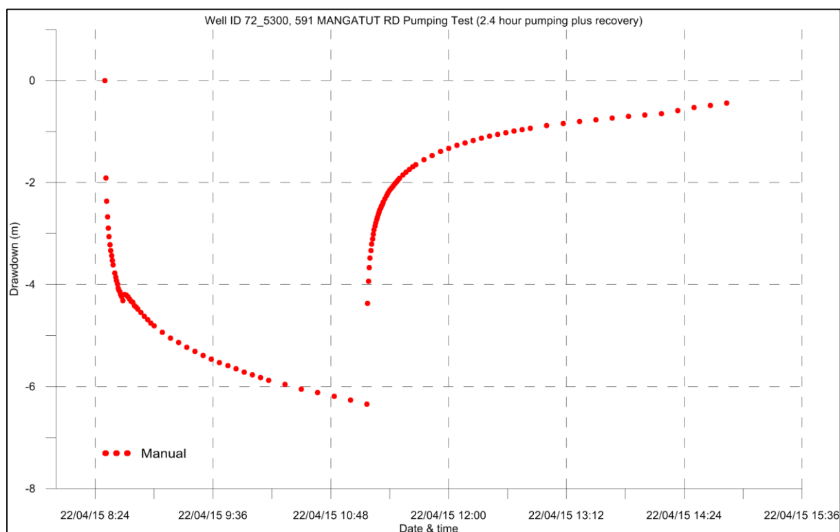
Figure A 3.17 Drawdown and recovery plot for well 72_5300.
