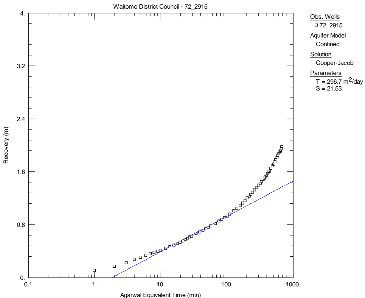
Figure A 3.6 Recovery data analysis for well 72_2915 fitting to the middle part of the curve, resulting in T = 296.7 \text{ m}^2/\text{day} .
