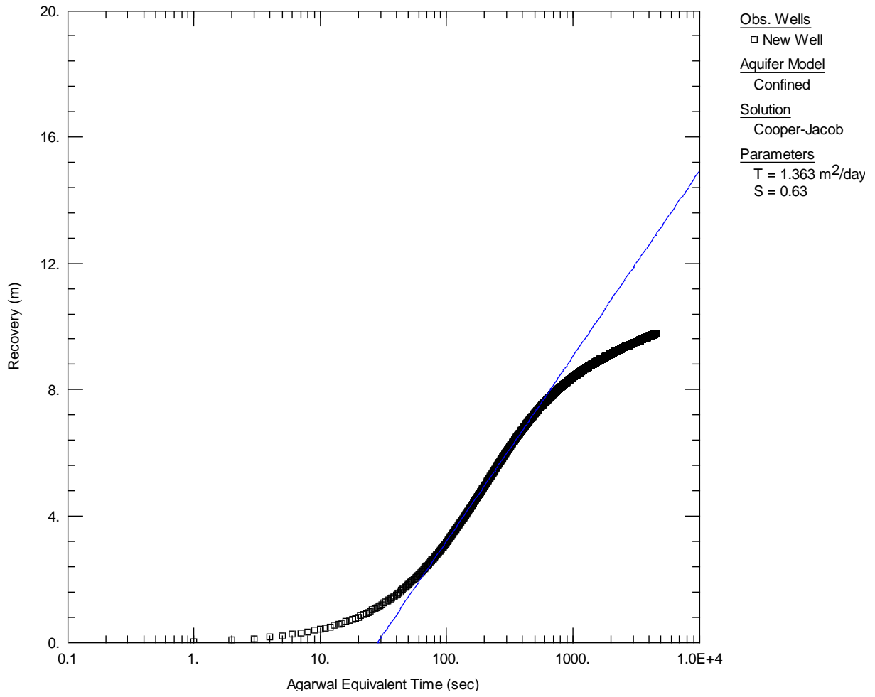
Figure A 3.2 Recovery data analysis for well 72_5569, resulting in T = 1.363 \text{ m}^2/\text{day} .
