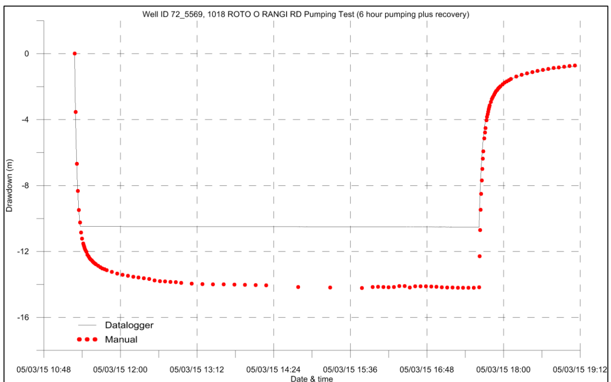
Figure A 3.1 Drawdown and recovery plot for well 72_5569.
