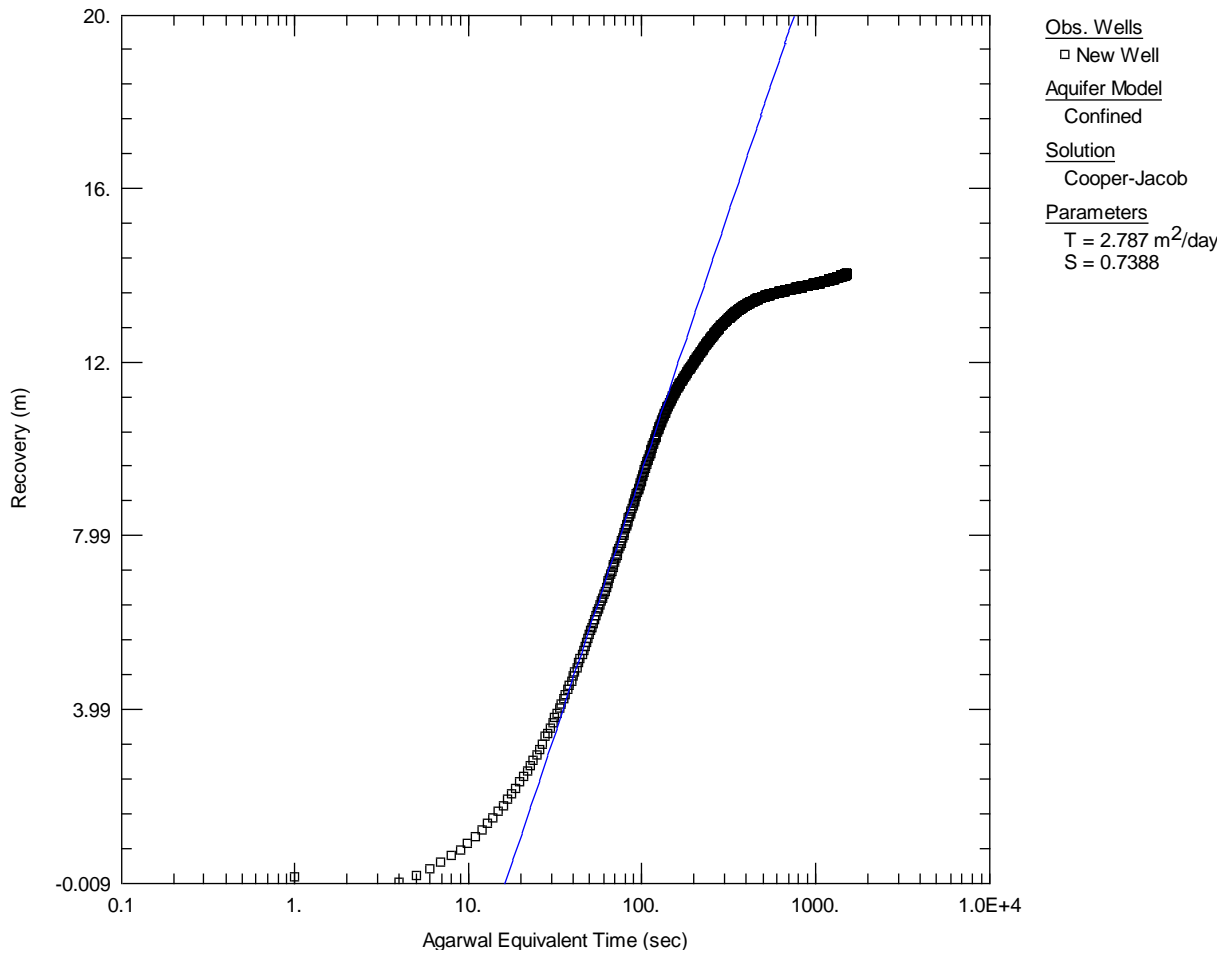
Figure A 3.20 Recovery data analysis for well 72_5009, resulting in T = 2.79 \text{ m}^2/\text{day} .
