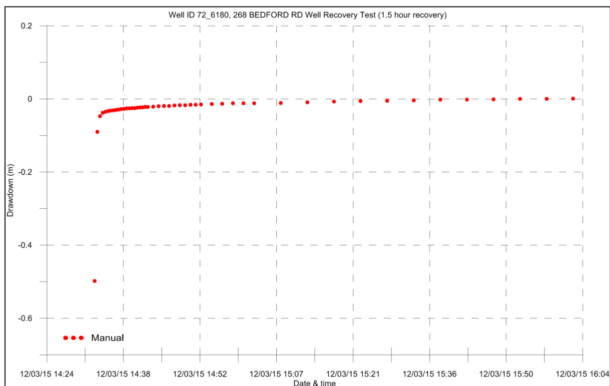
Figure A 3.3 Drawdown and recovery plot for well 72_6180.
