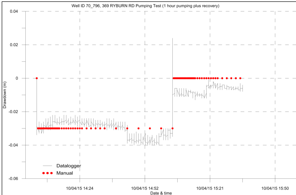
Figure A 3.21 Drawdown and recovery plot for well 70_796.
