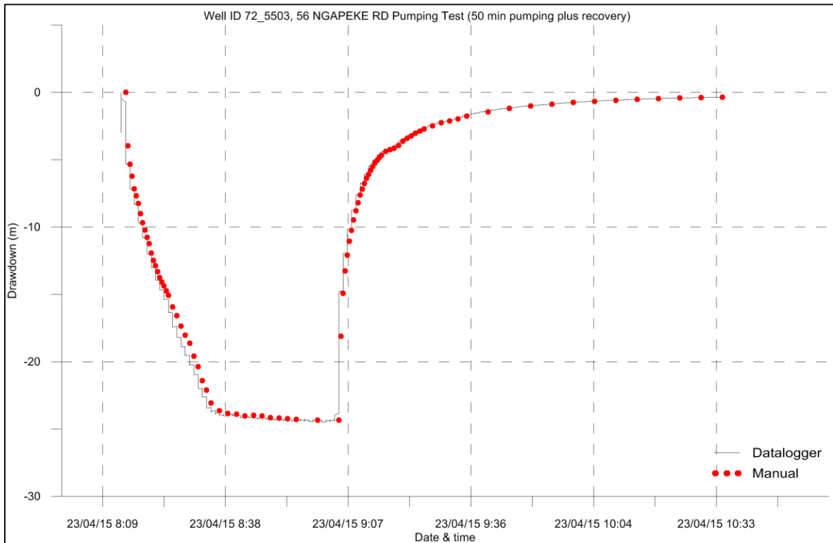
Figure A 3.11 Drawdown and recovery plot for well 72_5503.
