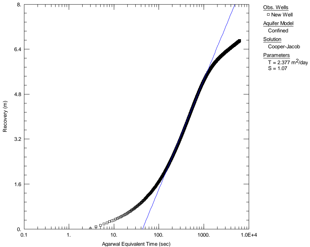
Figure A 3.16 Recovery data analysis for well 72_632, resulting in T = 2.38 \text{ m}^2/\text{day} .
