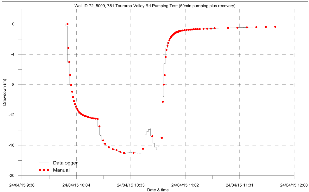
Figure A 3.19 Drawdown and recovery plot for well 72_5009.
