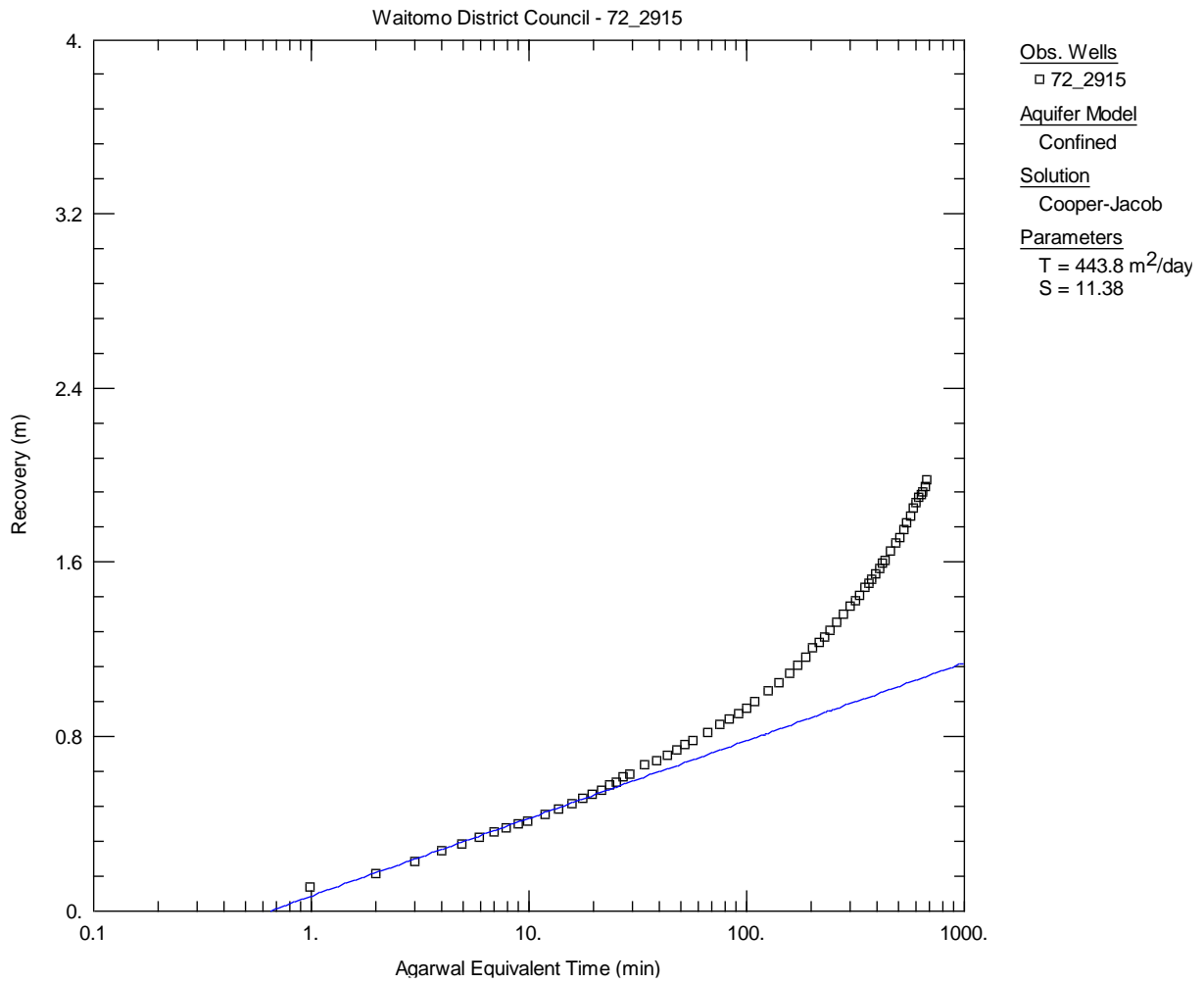
Figure A 3.7 Recovery data analysis for well 72_2915 fitting to the initial part of the curve, resulting in T = 443.8 \text{ m}^2/\text{day} .
