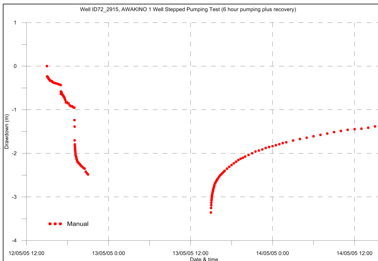
Figure A 3.5 Drawdown and recovery plot for well 72_2915.
