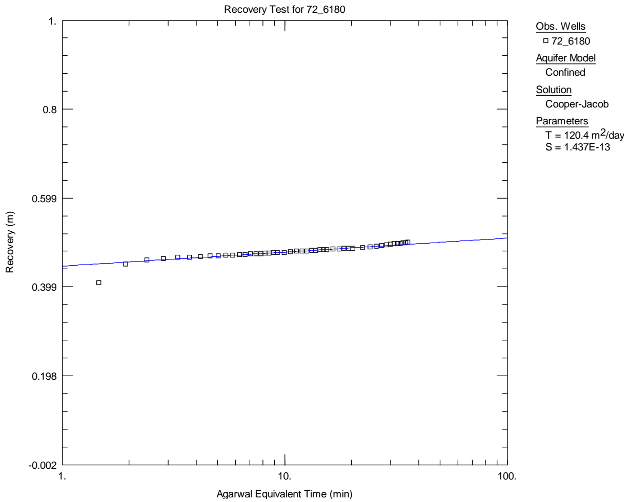
Figure A 3.4 Recovery data analysis for well 72_6180, resulting in T = 120.4 \text{ m}^2/\text{day} .
