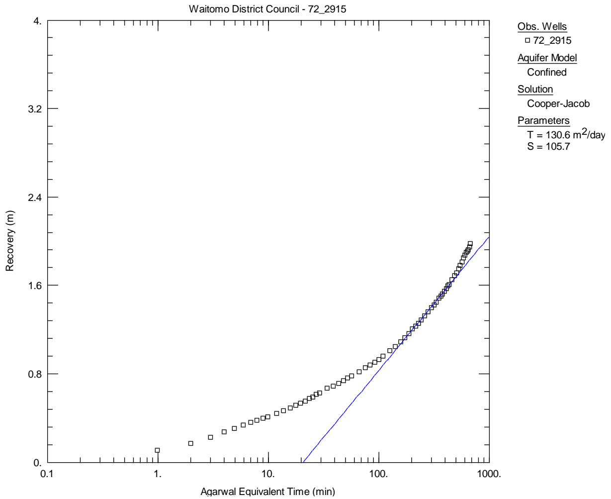
Figure A 3.8 Recovery data analysis for well 72_2915 fitting to the latter part of the curve, resulting in T = 130.6 \text{ m}^2/\text{day} .
