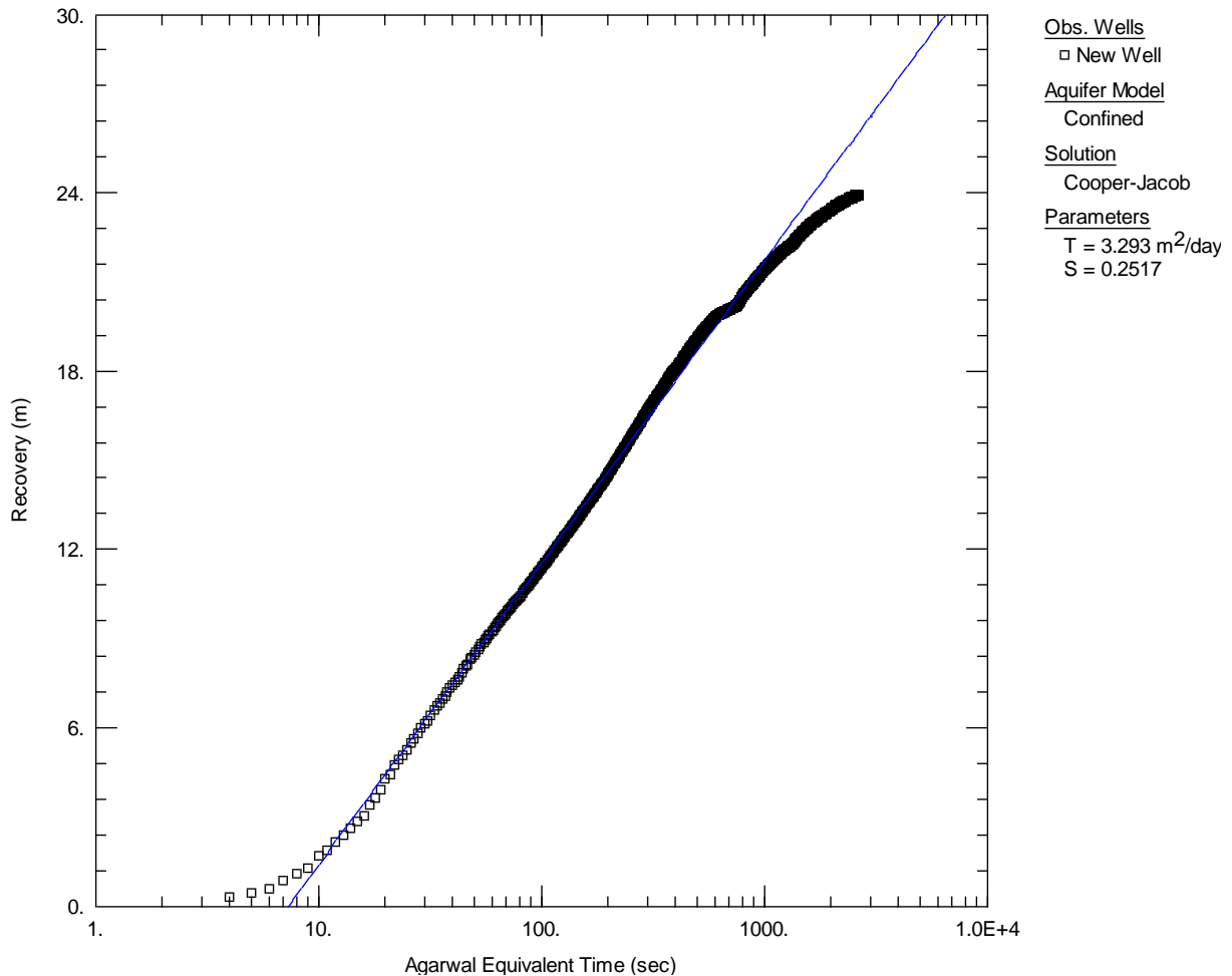
Figure A 3.12 Recovery data analysis for well 72_5503, resulting in T = 3.29 \text{ m}^2/\text{day} .
