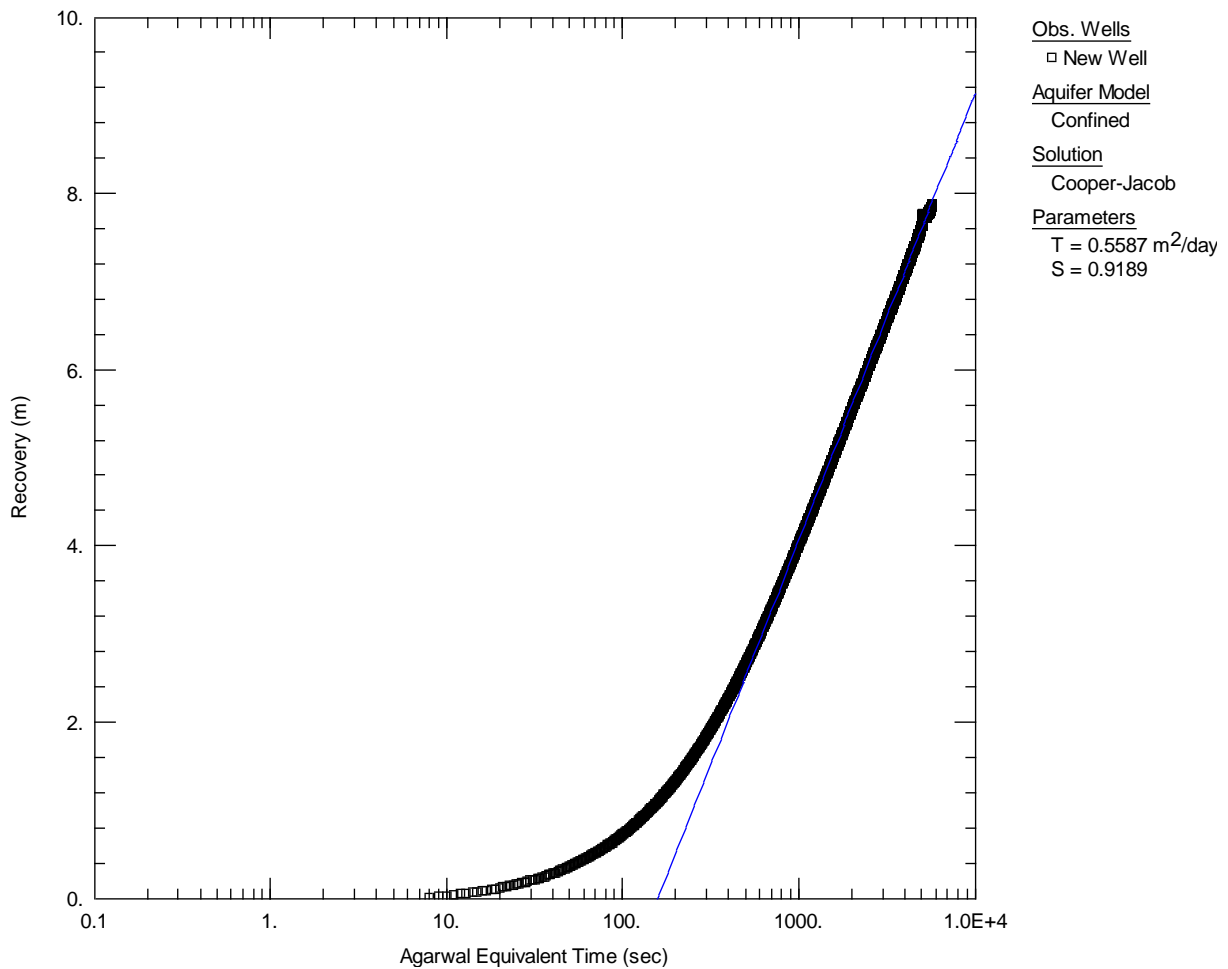
Figure A 3.14 Recovery data analysis for well 72_4759, resulting in T = 0.56 \text{ m}^2/\text{day} .
