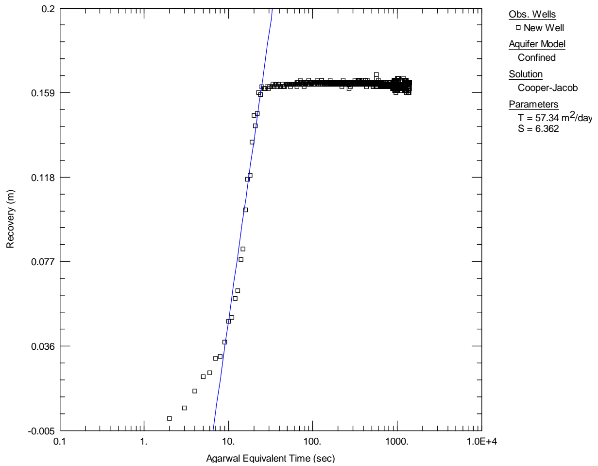
Figure A 3.10 Recovery data analysis for well 72_4014, resulting in T = 57.34 \text{ m}^2/\text{day} .
