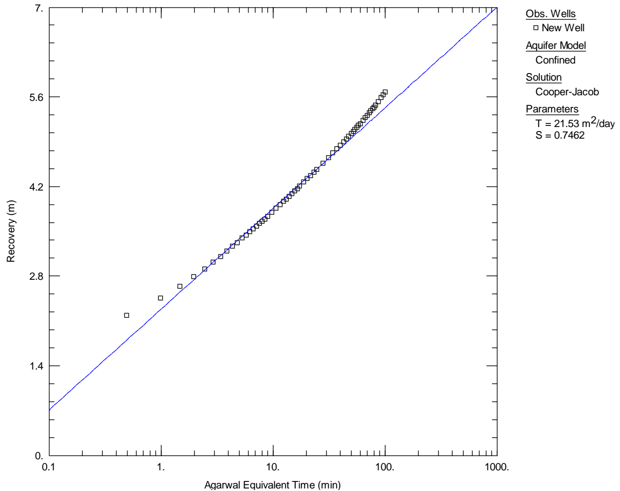
Figure A 3.18 Recovery data analysis for well 72_5300, resulting in T = 21.53 \text{ m}^2/\text{day} .
